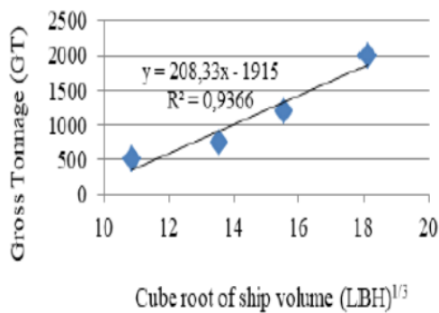
Fig. 6. The relation between nondimensional parameter of ship volume and gross tonnage
